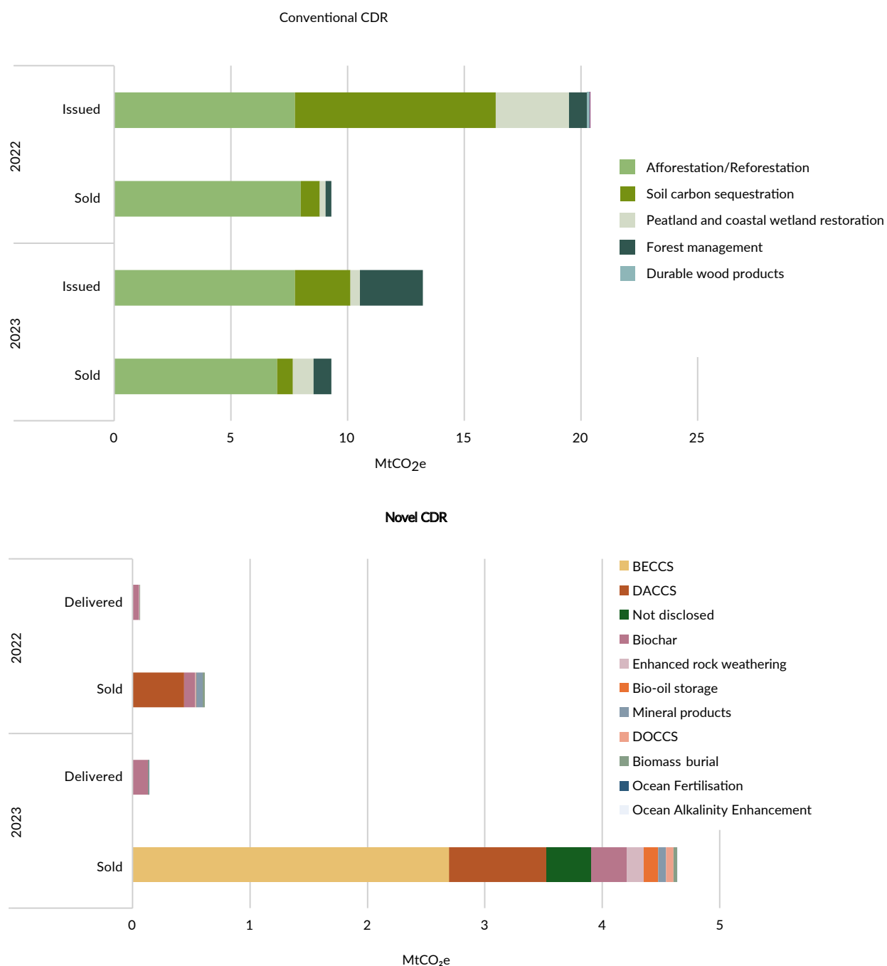
Figure 4.4 Breakdown of the volume of carbon dioxide removal (CDR) in the voluntary carbon market (VCM) by CDR method, 2022–2023. Top panel: conventional CDR; bottom panel: novel CDR. BECCS = bioenergy with carbon capture and storage; DACCS = direct air carbon capture and storage; DOCCS = direct ocean carbon capture and storage.
